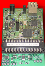
8ch 5Gbps-Digital Baseband Processor
